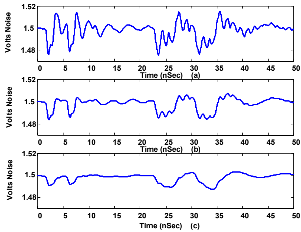
Figure 12. Simulated I/O noise for different dielectric thickness: (a) 2 mils: V_{pp}=39.9 mV (b) 1 mil: V_{pp}=23.4 mV (c) 0.5 mil: V_{pp}=15.8 mV
