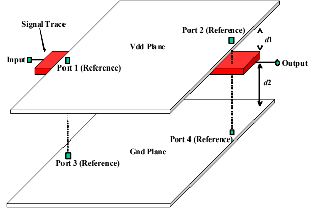
Figure 8. Transmission line between vdd/gnd planes
