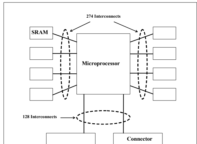
Figure 1. Top view of functioning board
